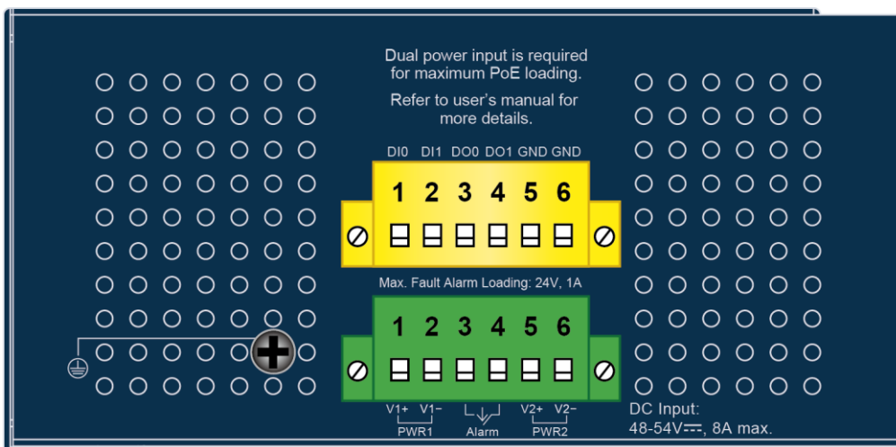
Figure 2-1-4b: Industrial Managed Switch Upper Panel.
