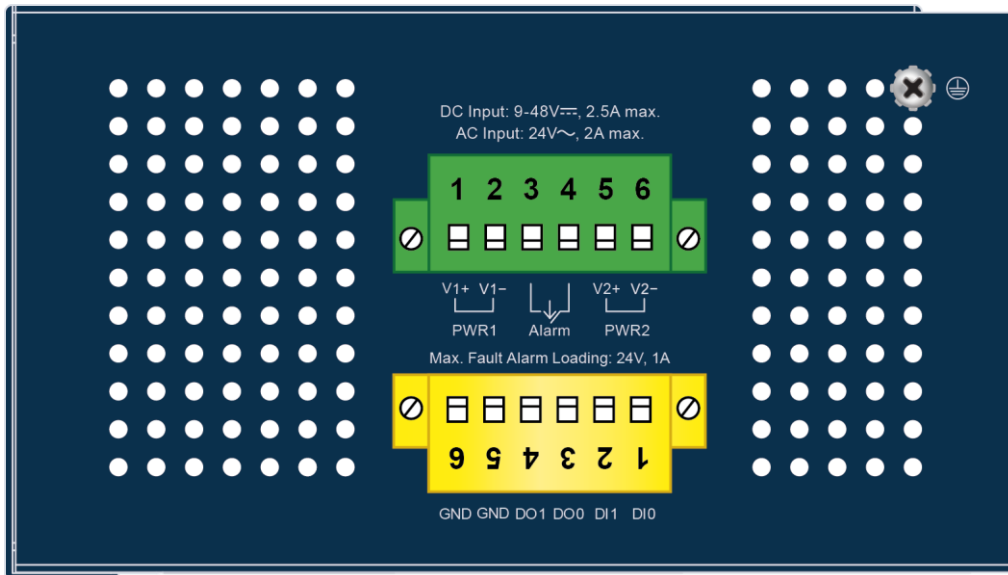
Figure 2-1-4c: Industrial Managed Switch Upper Panel
