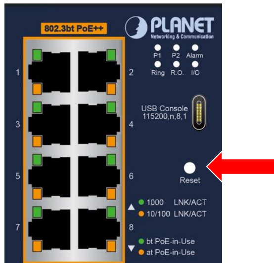
Reset button
