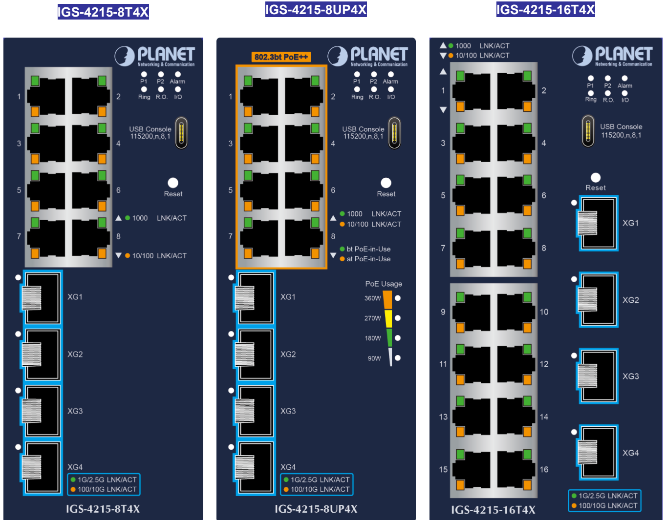
Figure 2-1-3a: IGS-4215-8T4X
